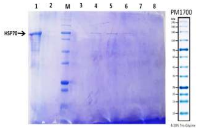
Fig. 3. Analysis of purification of rHSP70. Lane 1, soluble cell lysate before purification; lane 2, flow-through; lane M, protein molecular weight marker; lane 3, washed away proteins; lanes 4-7, eluted proteins; lane 8, MES buffer
