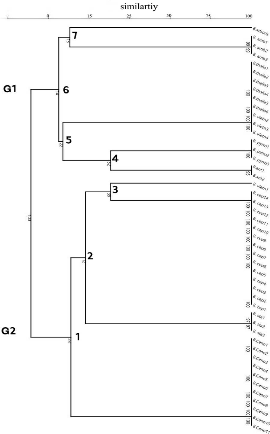
Fig. 2 . UPGMA dendrogram generated by BioNumerics software PAST showing the biochemical relationships among Bcc isolates
